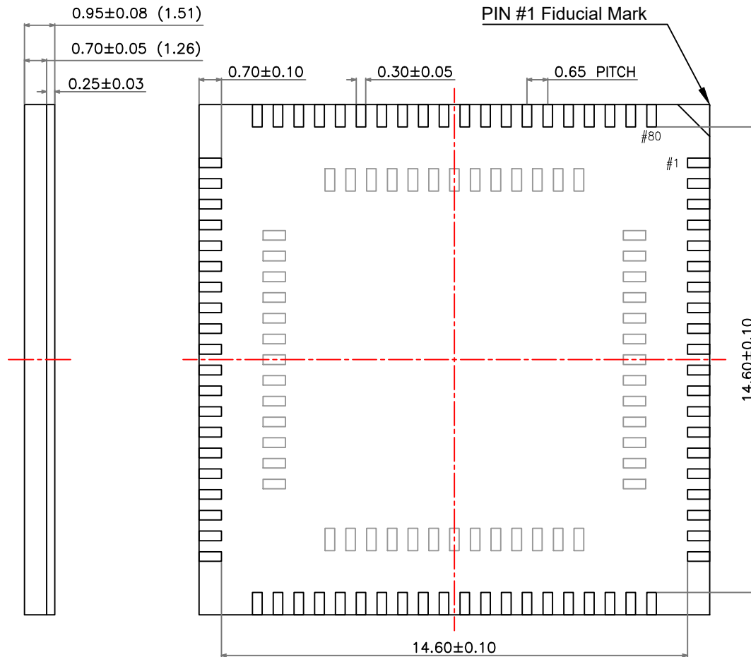
SIDE VIEW
